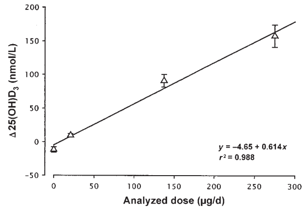
FIGURE 2. Regression of the equilibrium increment ( \Delta ) in serum 25-hydroxycholecalciferol [25(OH)D 3 ] concentration ( a , from Equation 1) on analyzed doses for the means of each treatment group.
