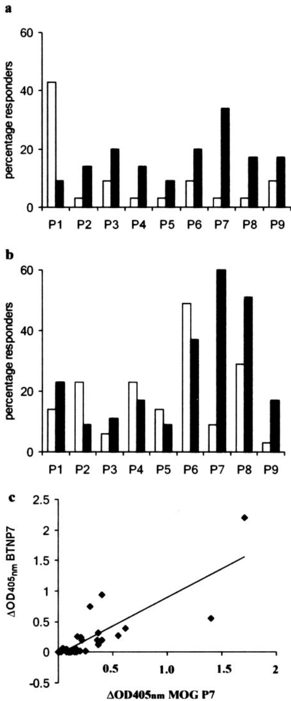
FIGURE 2. Differential patterns of epitope recognition in MS sera and CSF. The Ab response to BTN 1-26 (a) and MOG 14-39 (b) peptides was assayed in paired samples of MS sera (□) and CSF (■; n = 35 ). The bars represent the percentage of donors responding to each peptide. Note the high frequency of CSF responses to peptides spanning amino acid sequences 76–100 of both BTN 1-26 and MOG 14-39 . c, Comparison of Ab responses to MOG 76–100 and BTN 76–100 in CSF for all 35 MS patients ( R^2 = 0.681 ). Data are presented as the mean OD corrected for background obtained from samples assayed in quadruplicate.
